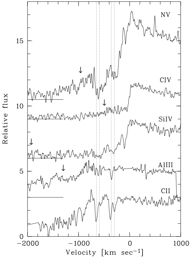
Fig. 2. Profiles of the red edges of several resonance-line absorption troughs. The velocity scale assumes a systemic redshift of 2.6327. In the case of doublets the velocity refers to the red doublet component. The ( v = 0 ) positions of the blue doublet components are indicated by vertical arrows. In the case of C II the velocity scale corresponds to the mean wavelength of the two fine structure components C II* \lambda\lambda 1335.66, 1335.71 of C II (UV1). Features caused by the ground state \lambda 1334.53 line of this multiplet are shifted (by about 260 km s -1 ) to apparently more negative velocities. As a result the -360 km s -1 component of the 1334.53 Å line overlaps with the -650 km s -1 component of C II*, while the -650 km s -1 feature of the 1334.53 line occurs at the apparent velocity -910 km s -1 . The apparent common absorption features mentioned in the text are indicated by dotted vertical lines.
