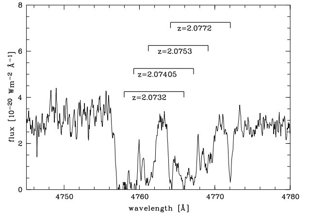
Fig. 3. Profile of the complex 2.0729 < z < 2.0772 foreground C IV doublet absorption system.
