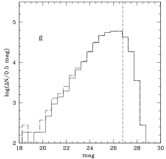
Fig. 7. Galaxy number counts of the FDF in g band (not corrected for incompleteness). The vertical dash-dotted line indicates the 50% completeness limits.
