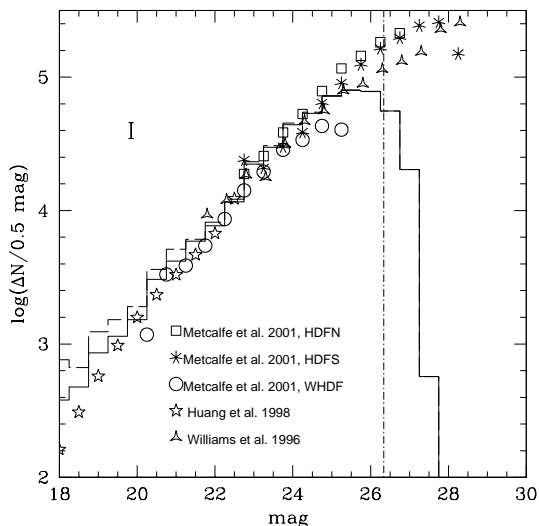
Fig. 9. Galaxy number counts of the FDF in I band (not corrected for incompleteness) as compared to other deep surveys. The vertical dash-dotted line indicates the 50% completeness limits.
