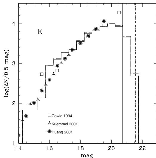
Fig. 11. Galaxy number counts of the FDF in Ks band (not corrected for incompleteness) as compared to other deep surveys. The vertical solid line indicates the 50% completeness for the shallower exposed part of the field, whereas the vertical dash-dotted line indicates the 50% completeness for the deeply exposed part of the field.
