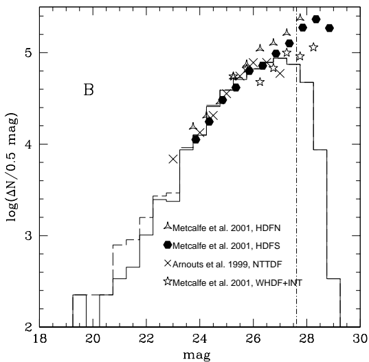
Fig. 6. Galaxy number counts of the FDF in B band (not corrected for incompleteness) as compared to other deep surveys. The vertical dash-dotted line indicates the 50% completeness limits.
