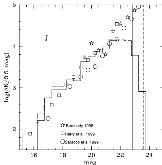
Fig. 10. Galaxy number counts of the FDF in J band (not corrected for incompleteness) as compared to other deep surveys. The vertical solid line indicates the 50% completeness for the shallower exposed part of the field, whereas the vertical dash-dotted line indicates the 50% completeness for the deeply exposed part of the field.
