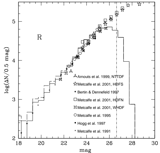
Fig. 8. Galaxy number counts of the FDF in R band (not corrected for incompleteness) as compared to other deep surveys. The vertical dash-dotted line indicates the 50% completeness limits.
