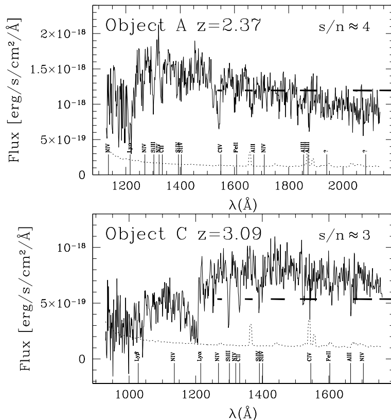
Fig. 4. Spectra of objects A (top panel) and C (lower panel), which lie \approx 20'' SW and \approx 10'' NE of the arc, respectively. \text{Ly}\alpha absorption and metal lines are indicated as in Figure 2.
