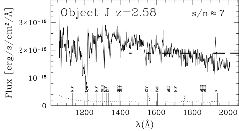
Fig. 5. Spectrum of object J, which lies \approx 2.5' SW of the arc. \text{Ly}\alpha absorption and metal lines are indicated as in Figure 2.
