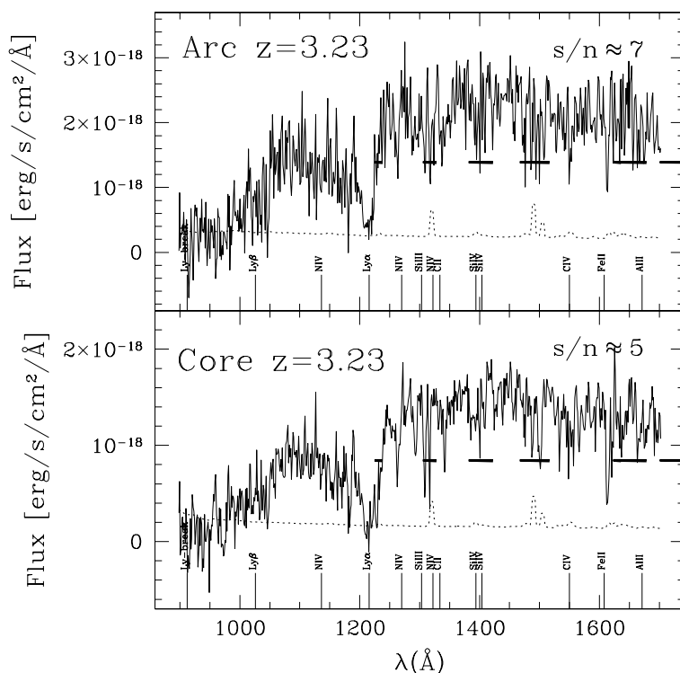
Fig. 2. Flux calibrated spectra of the arc ( 10'' , top panel) and the core ( 3'' , lower panel). The \text{Ly}\alpha absorption line as well as the position of expected metal absorption lines are indicated. The horizontal bars indicate the position of prominent night sky blends (blueshifted to the rest frame of the galaxy). The dotted lines indicate the size of the 1\sigma error level of the flux.
