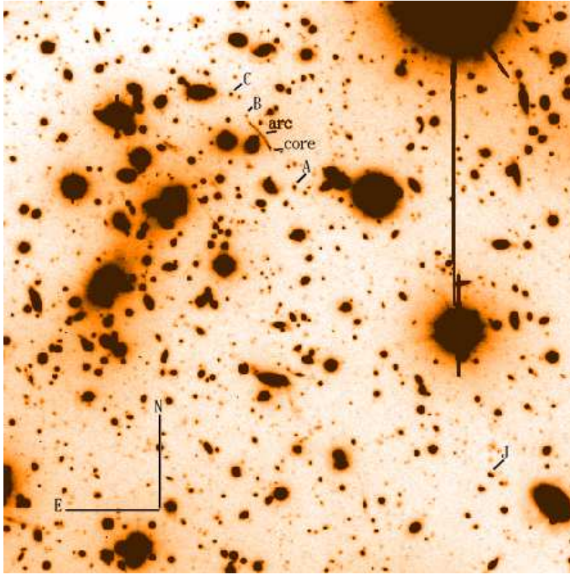
Fig. 1. R-band image of the galaxy cluster 1E 0657 taken during the commissioning of FORS in December 1998 (field of view (FOV) = 3.2' \times 3.2' ; 0.2'' per pixel; exposure time = 3 \times 600 s; seeing = 0.65'' \dots 0.8'' ). The positions of the arc and some other objects (see Section 3) are indicated. North on the top, East to the left.
