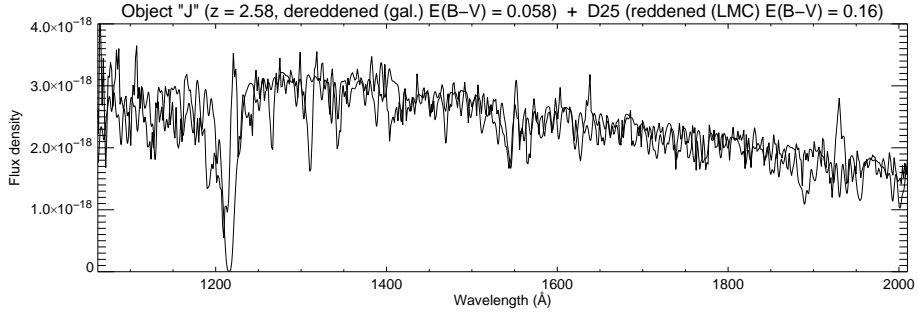
Fig. 6. Comparison of object J (thin line) and a synthetic spectrum (thick line). (See text).
