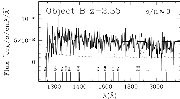
Fig. 3. Spectrum of Object B, which lies a few arcsec NE of the arc. \text{Ly}\alpha absorption and metal lines are indicated as in Figure 2. The horizontal bars and dotted lines have the same meaning as in Figure 2.
